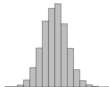
Normal distribution
